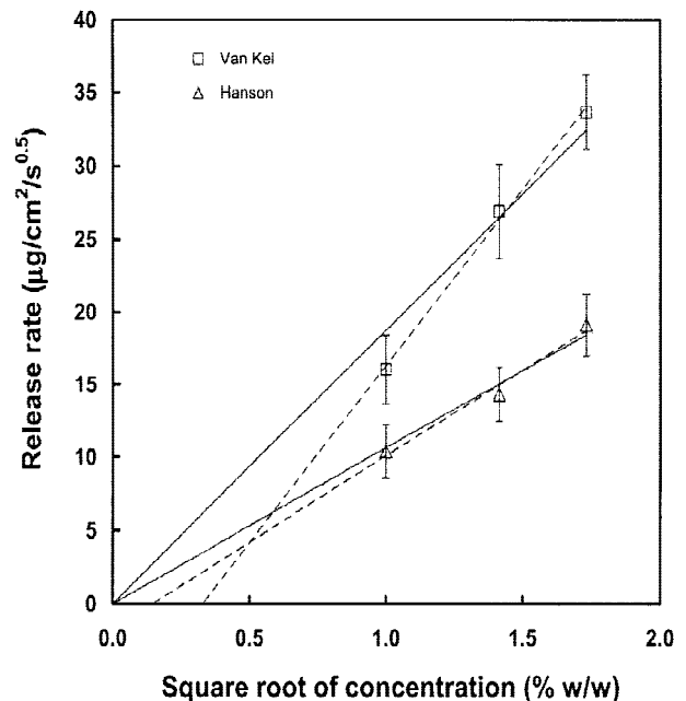
Fig. 4. Comparison of average slopes obtained with formulations containing 1%, 2% and 3% E232 vs. square root of concentration (% w/w), using SD as error bars. Dashed lines (---) show the Y = m \cdot x + b regression fit for the Hanson ( R^2 = 0.983 ) and Van Kel ( R^2 = 0.997 ) apparatus. Continuous lines (—) illustrate the Y = m \cdot x regression fit for the Hanson ( R^2 = 0.972 ) and Van Kel ( R^2 = 0.944 ) apparatus.
